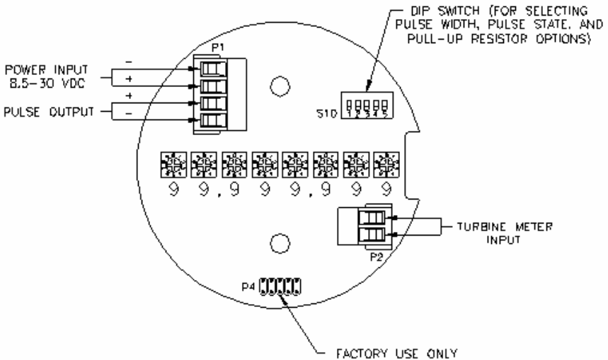
Figure 1 Terminal Connections
